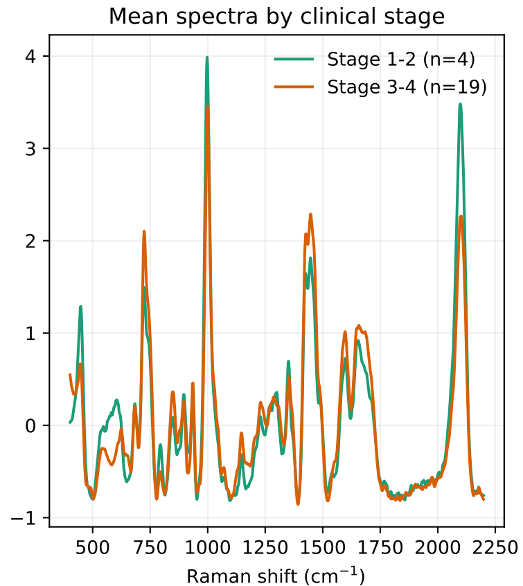
Fig05. Severance pancreatic cancer internal subgroup check by stage
